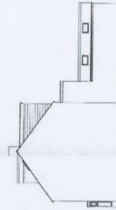
Existing Side Elevation
